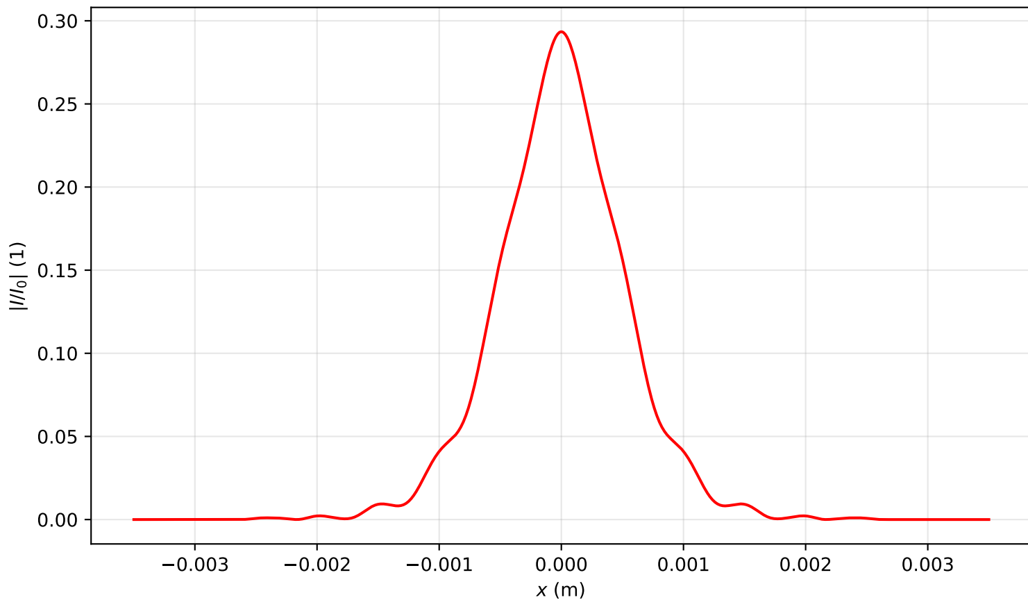
Intensity profile I(x, y = 0, z = 3.184)/I_0 , P_{in}=1.0P_{cr} , artificial time
